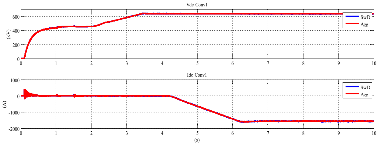
Figure 6. Generated DC voltage & DC current
