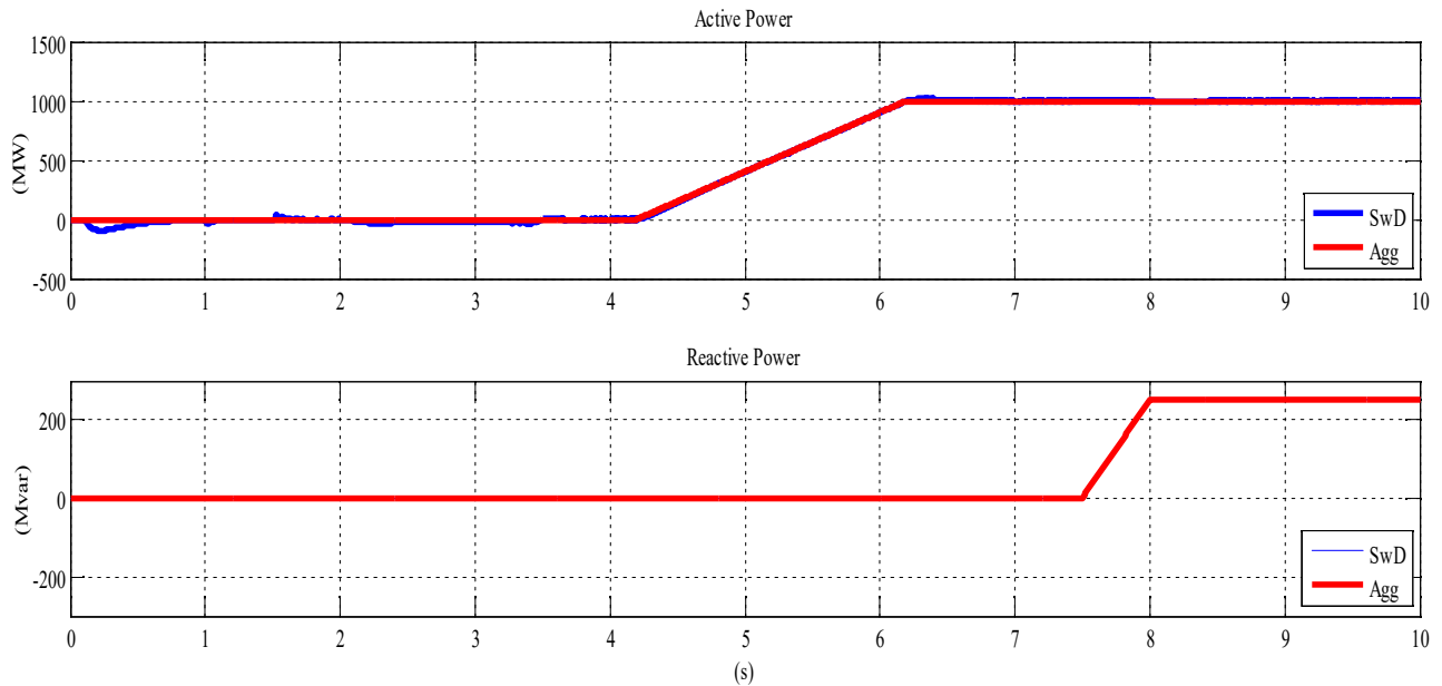
Figure 7. Active power & reactive power
