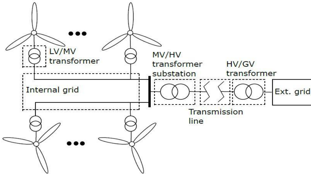
Figure 2. OWF arrangement.
